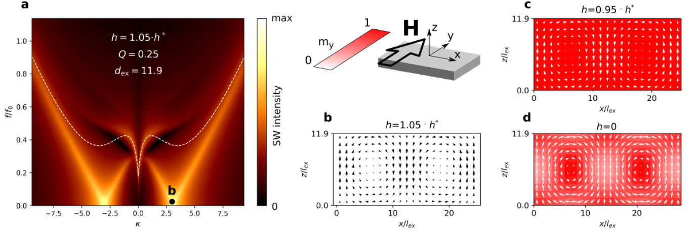
FIG. 4. Simulated h -dependent static and dynamic properties of thin film with Q = 0.25 , D_{\text{ex}} = 0 , and d_{\text{ex}} = 11.9 . (a) SW dispersion relation for h = 1.05 \cdot h^* (SW intensity is in log scale); the white dashed line represents the analytical dispersion (Eq. 1); (b) mode of oscillations at the point (\kappa_{\text{min}}, f_{\text{min}}) in the dispersion relation, as marked with the black dot in (a); the m_x and m_z dynamic magnetization components are presented by the black arrows, m_y \approx 1 ; (c, d) static magnetization distribution at h = 0.95 \cdot h^* and h = 0 , respectively. The m_x and m_z static magnetization components are presented by the white arrows, the static m_y component is coded by color.
