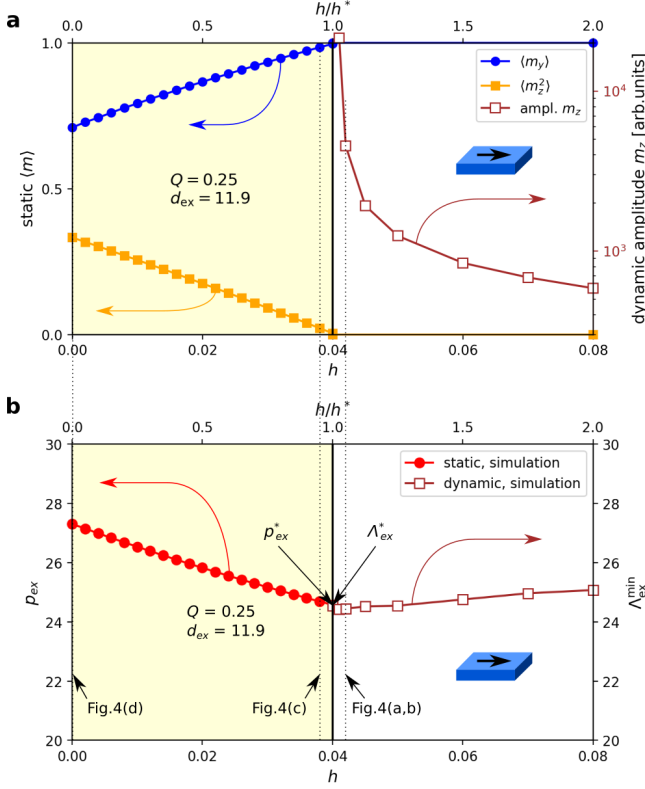
FIG. 8. A relation between the static magnetization configuration of stripe domain pattern and the SW profile below and above SRT, respectively. Simulations have been performed for the thin film depending on h for d_{ex} = 11.9 , Q = 0.25 , and D_{ex} = 0 . Normalized field h -dependencies are of the following: (a) static \langle m_y \rangle and \langle m_z^2 \rangle (solid squares and circles); critical field h^* = 0.04 is determined by simulations; maximal amplitude of oscillations in determined by dynamic simulations (open squares); (b) reduced equilibrium domain period p_{ex} is determined by static simulations (solid circles) and wavelength of SWs \Lambda_{ex}^{min} is determined by dynamic simulations (open squares). Solid lines are plotted as guides for the eye. The yellow background corresponds to the field range of occurrence of magnetic state with out-of-plane magnetization component, while the white background corresponds to the in-plane state.
