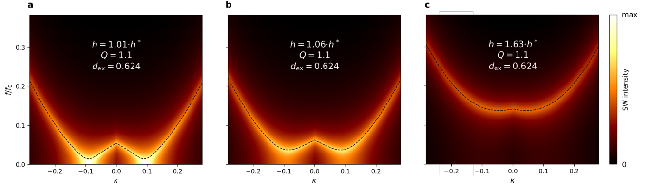
FIG. 7. Dispersion relation in ultrathin film for d_{\text{ex}} = 0.624 (i.e., 2 nm of Co), Q = 1.1 , D_{\text{ex}} = 0 , and increasing field, all above the critical value h^* = 0.123 : (a) h = 1.01 \cdot h^* ; (b) h = 1.06 \cdot h^* (this is the case presented in Fig. 1(a)); (c) h = 1.63 \cdot h^* . SW intensity is coded by color in log scale. While increasing the field, the band moves up and its intensity decreases. The dashed lines are plotted according to the dispersion-based theory (Eq. 1).
