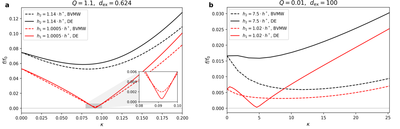
FIG. 11. The simulated dispersion relations in DE (solid lines) and BVMW (dashed lines) modes for the two following systems: (a) an ultrathin film, d_{\text{ex}} = 0.624 and Q = 1.1 , and in magnetic field, h_1 = 1.0005 \cdot h^* and h_2 = 1.14 \cdot h^* ; (b) a thick and low-anisotropy film, Q = 0.01 and d_{\text{ex}} = 100 , and in magnetic field, h_1 = 1.02 \cdot h^* and h_2 = 7.5 \cdot h^* .
