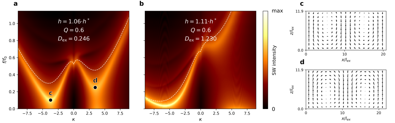
FIG. 10. Dispersion relations and SW mode profiles in thin film with DMI, d_{\text{ex}} = 11.9 and Q = 0.6 . (a, b) Dispersion relations for D_{\text{ex}} = 0.246 and D_{\text{ex}} = 1.23 and h = 1.06 \cdot h^* and h = 1.11 \cdot h^* , respectively. While increasing DMI the band tilts, becoming more asymmetric. SW intensity is coded by color in log scale. The white dashed lines are theoretical dependences according to Eq. 1 at the given values of field. (c, d) Mode profiles for D_{\text{ex}} = 0.246 in h = 1.06 \cdot h^* , at the points marked with dots in (a).
