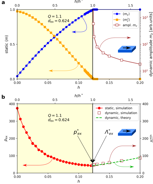
FIG. 2. A relation between the static magnetization configuration of stripe domain pattern and the SW profile, below and above SRT, respectively. Simulations have been performed for an ultrathin film depending on h for d_{\text{ex}} = 0.624 , Q = 1.1 , and D_{\text{ex}} = 0 . Normalized field h -dependencies are of the following: (a) static \langle m_y \rangle and \langle m_z^2 \rangle (solid circles and squares); critical field h^* = 0.123 is determined by simulations; maximal amplitude of m_z oscillations from dynamic simulations (open squares); (b) reduced equilibrium domain period p from static simulations (solid circles), SW wavelength \Lambda_{\text{ex}}^{\text{min}} from dynamic simulations (open squares), and from theory given by Eqs. 1 and 2a (dashed green line). Solid lines are plotted as guides for the eye. The yellow background corresponds to the field range of occurrence of magnetic state with out-of-plane magnetization component, and the white background corresponds to in-plane state.
