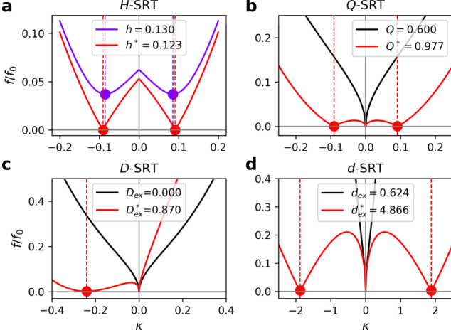
FIG. 1. Analytical dispersion relations constructed with Eq. 1 illustrating conditions required for SRT occurrence. (a) H -SRT for Q = 1.1 , D_{\text{ex}} = 0 , and d_{\text{ex}} = 0.624 ; (b) Q -SRT for h = 0 , D_{\text{ex}} = 0 , and d_{\text{ex}} = 0.624 ; (c) D -SRT for h = 0 , Q = 0.6 , and d_{\text{ex}} = 0.624 ; (d) d -SRT for h = 0 , Q = 0.6 , and D_{\text{ex}} = 0 . Black lines in (b)–(d) concern the same set of parameters ( h = 0 , Q = 0.6 , D_{\text{ex}} = 0 , d_{\text{ex}} = 0.624 ). The red dots and vertical dashed lines represent the conditions, where Eqs. 2a and 2b are satisfied, indicating the values of \kappa^* . The violet dots in (a) represent the conditions, where only Eq. 2a is satisfied.
