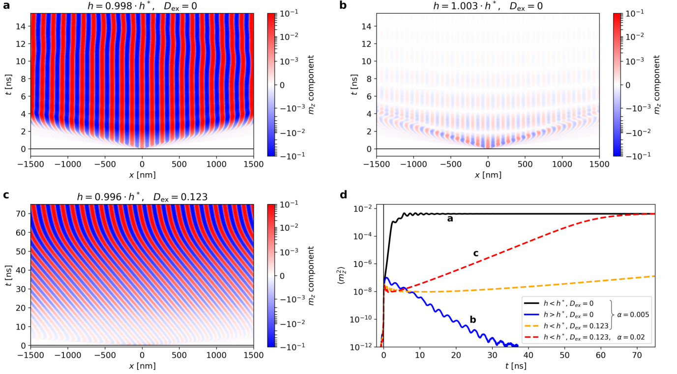
FIG. 3. Time evolution of the pattern formation in ultrathin Co film for Q = 1.1 . (a) h = 0.998 \cdot h^* and (b) h = 1.003 \cdot h^* ; in these simulations, h^* = 0.123 , D_{\text{ex}} = 0 , and damping parameter \alpha = 0.005 . (c) D_{\text{ex}} = 0.123 , h = 0.996 \cdot h^* (where h^* = 0.124 ), and \alpha = 0.02 . The color scales in all density maps are conserved. (d) Temporal dependencies of \langle m_z^2 \rangle are averaged over the whole systems, for the cases (a), (b), and (c), and additionally for the DMI case from (c) with low \alpha = 0.005 (the orange dashed line). The same results in the form of a movie can be found in Supplemental Material [41].
