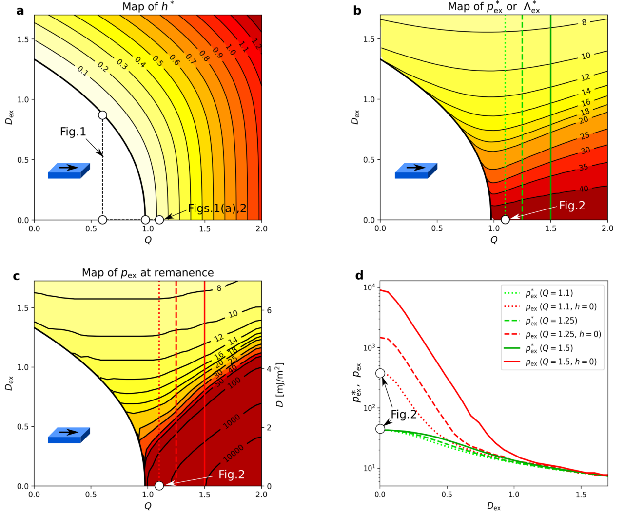
FIG. 5. Calculated diagrams and SRT lines in the (Q, D_{\text{ex}}) space for the ultrathin film case with d_{\text{ex}} = 0.624 . (a, b) Theoretical SRT (i.e., numerical solution of Eqs. 2a and 2b); (a) the map of critical field h^* ; (b) the map of critical period p_{\text{ex}}^* or wavelength \Lambda_{\text{ex}}^* for the values of h^* shown in (a); (c) the map of reduced period found in micromagnetic simulations from energy minimization at zero field; (d) a comparison of freezing (b) and zero-field (c) reduced periods for selected Q values (marked with the vertical lines in (b) and (c)). The white points denote the parameters discussed in the labelled figures.
