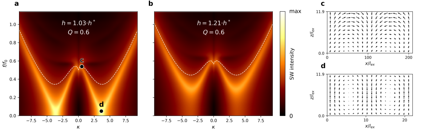
FIG. 9. Dispersion relations and SW mode profiles in thin films, d_{\text{ex}} = 11.9 and Q = 0.6 . (a, b) Dispersion relations for h = 1.03 \cdot h^* and h = 1.21 \cdot h^* . While increasing the field above the band moves up and its intensity decreases. SW intensity is coded by color in log scale. The white dashed lines are theoretical dependences according to Eq. 1 at the given values of field. (c, d) Mode profiles in h = 1.03 \cdot h^* , where h^* = 0.32 , at the points marked with dots in (a).
